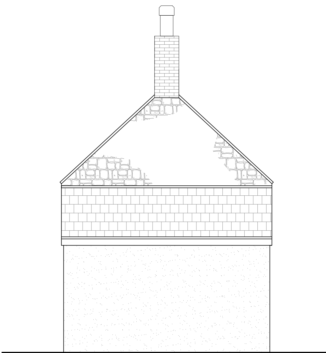
EXISTING WEST FACING ELEVATION SCALE 1/50
